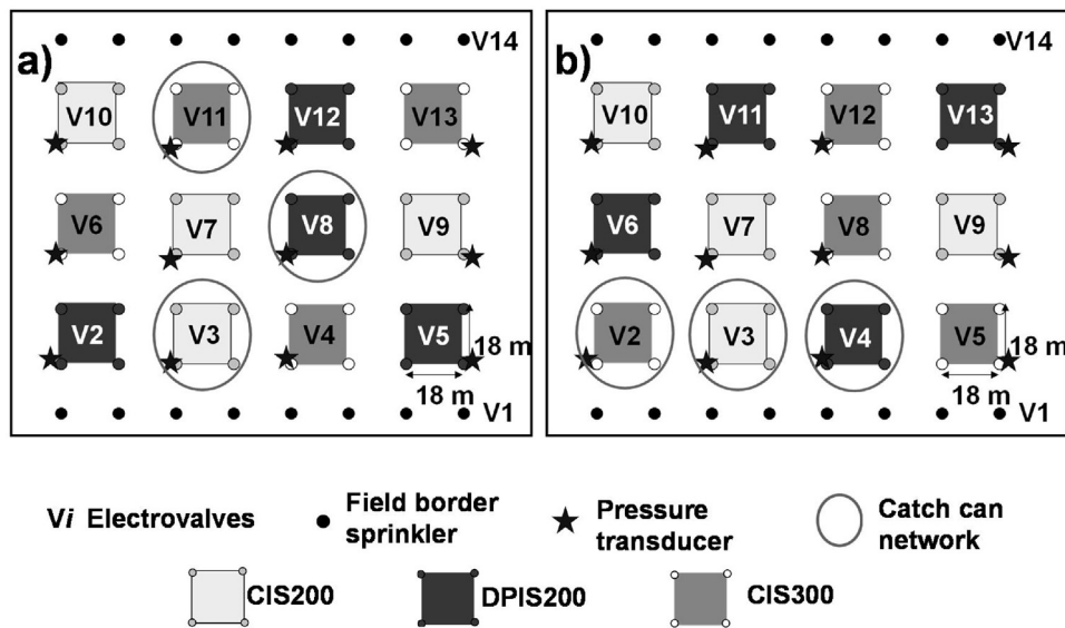
Fig. 1. Experimental design configuration, location of the three treatments and four replicates in 2015 season (Fig. 1a) and in 2016 season (Fig. 1b). Treatments are: CIS300, standard pressure treatment; CIS200, low pressure treatment; and DPIS200, low pressure treatments with modified sprinkler. Location of the pressure transducer in each experimental plot and the experimental plots selected for catch-cans evaluation in each season are also shown.
