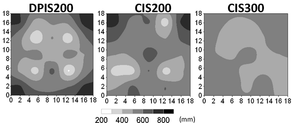
Fig. 7. Water distribution pattern of the accumulated irrigation applied in 2016 to one replicate of each treatment: DPIS200 (a), CIS200 (b) and CIS300 (c).
