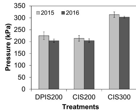
Fig. 4. Seasonal average of the water pressure measured with the pressure transducer at the sprinkler riser for each treatment during the 2015 and 2016 irrigation seasons. Error bars represents one standard deviation.
