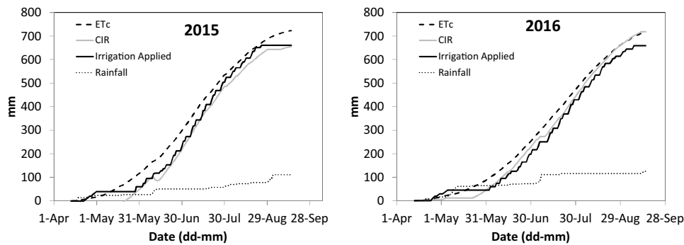
Fig. 3. Cumulative calculated crop evapotranspiration (ETc), rainfall, crop irrigation requirement (CIR) and irrigation applied water as a function of time during the season 2015 and 2016.
