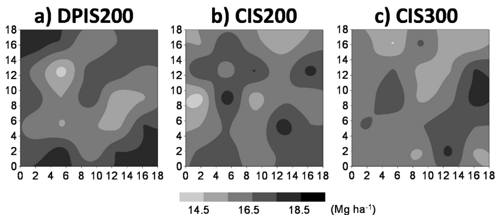
Fig. 8. Spatial variability of grain yield obtained by the intensive hand harvest performed in one replicate of each treatment: DPIS200 (a), CIS200 (b) and CIS300 (c), in 2016 crop season.
