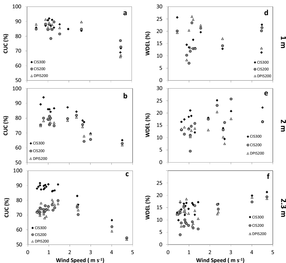
Fig. 5. Relationships between wind speed and uniformity coefficient, CUC, (a, b and c) and between wind speed and wind drift and evaporation losses, WDEL, (d, e and f) for each treatment and catch-cans elevation (1 m, 2 m and 2.3 m). Data presented for 1 m catch-cans elevation correspond to irrigations evaluated in 2015 and 2016 (a and d). Data for the other catch-cans elevation correspond only for irrigations evaluated in 2016.
