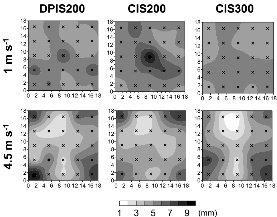
Fig. 6. Water distribution patterns of two individual irrigation events, one under low wind speed (upper figures) and the other under high wind speed conditions (lower figures), for the three treatments.
