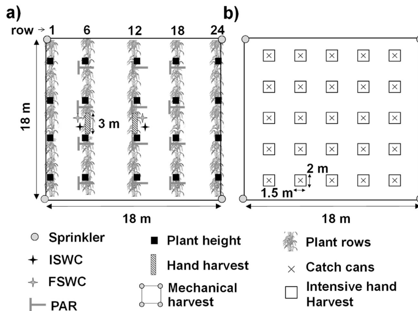
Fig. 2. Location of the measurement points for plant height, photosynthetically active radiation intercepted by the crop (PAR) and hand harvest for biomass and yield components determination at each experimental plot (Fig. 2a). Arrangement of the 25 catch-cans network and intensive hand harvest area at the three experimental plots were irrigation uniformity and yield variability was measured, was also presented (Fig. 2b).
